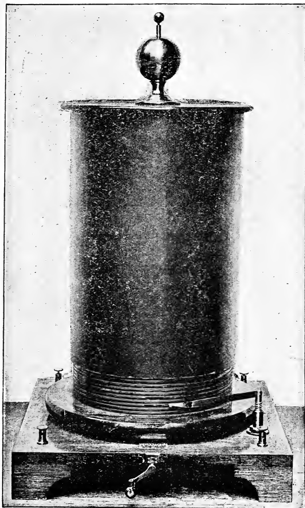
FIG. 49.—AUDIN'S RESONATER.
